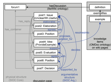
Figure 6: RDF Graph of a Discussion Thread about a Mathematical Definition (using our STEM-specific argumentation ontology)
